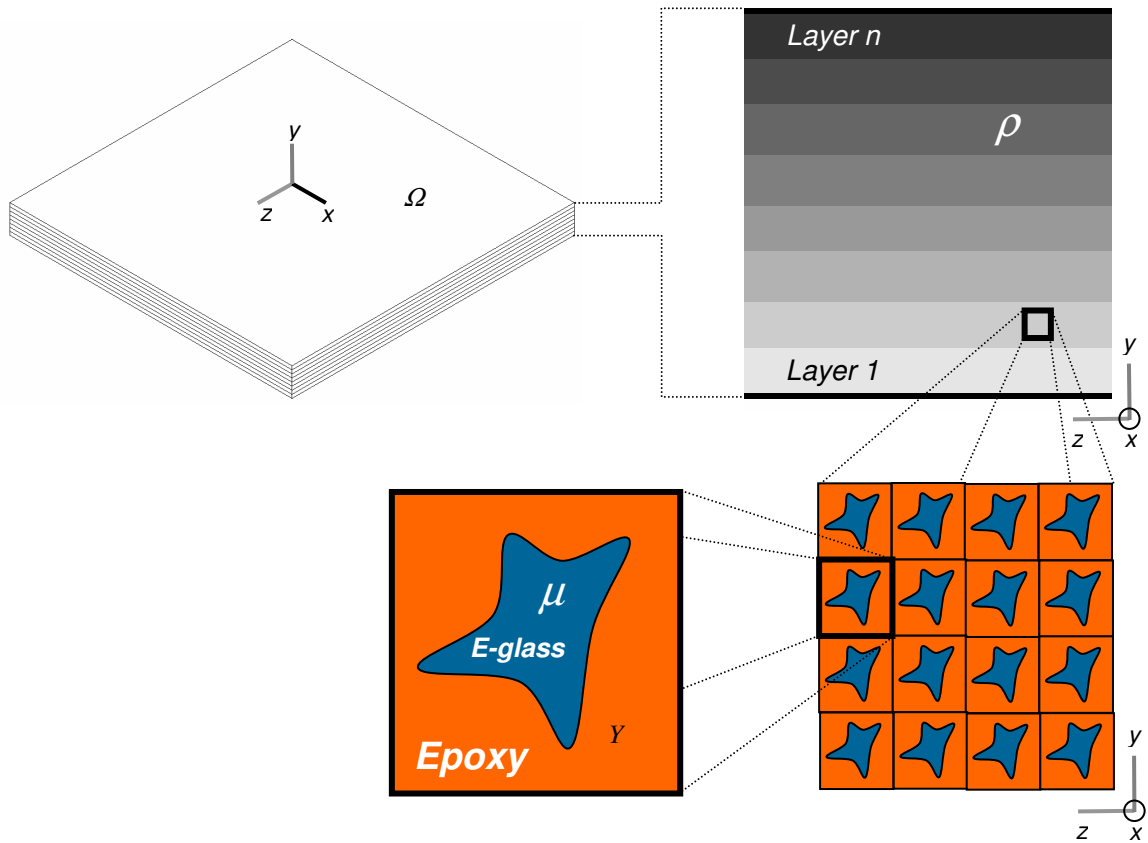
Figure 3: Bi-material interpolation scheme.
