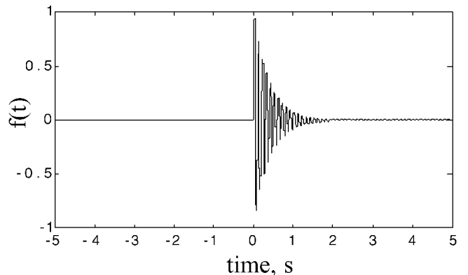
Fig. 4 Test signal (from Freidinger et al. 5 ).
