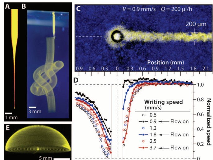
Fig. 2. Stable writing in the granular gel medium. (A) Injection tip filled with fluorescent microspheres suspension, imaged under UV illumination. (B) The tip revisits the same points in space hundreds of times with intermittent injection to create a continuous knot written with aqueous fluorescent microspheres suspension in aqueous granular gel (UV illumination, side and top views). (C) Writing structures atop a fluorescence microscope during live imaging allows a detailed study of yielding length scales and time scales. (D) The granular gel flow speed along the axis of translation is plotted normalized by the translation speed. Disturbances in flow decay within less than one tip diameter (see fig. S2). (E) A hemispherical cap made from uncrosslinked 1- \mu\text{m} microspheres, created 6 months before photographing, exhibits long-term stability provided by the granular gel medium.
