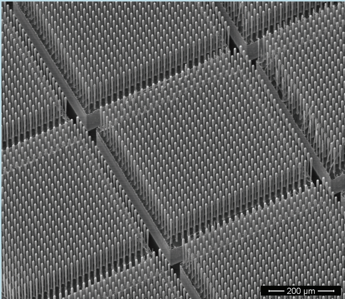
Saeed Moghaddam's group is developing hierarchical micro/nano-structured devices to enhance phase-change heat transfer.
