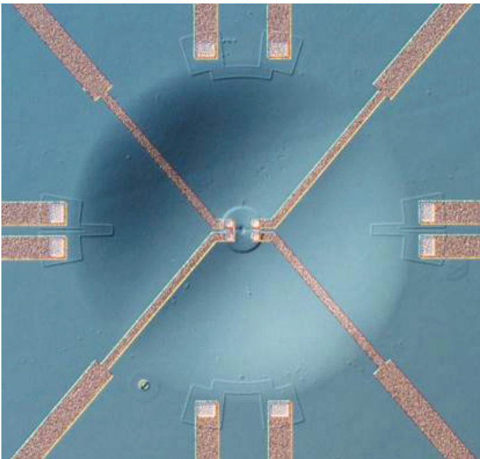
Micromachined acoustic proximity sensor from Venkat's dissertation work.
