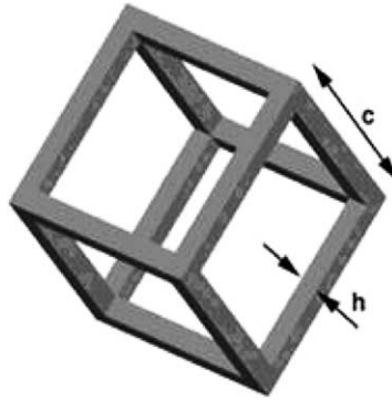
Fig. 2. Open rectangular cell model. The uni-cell is assumed to be a cube of dimension c and the struts (cell edges) are assumed to have a square cross-section h \times h .
