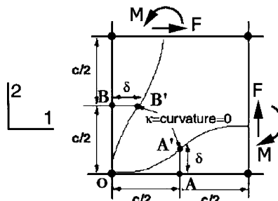
Fig. 4. Deformed shape of struts in an open-cell foam subjected to uniform macroscale shear stresses.
