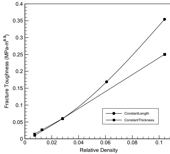
Fig. 15. Mode II fracture toughness as a function of relative density for two cases: constant unit-cell length (200 μm) and constant strut thickness (20 μm).
