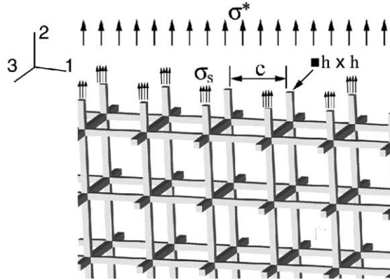
Fig. 3. The cellular medium subjected to a uniform macrostress \sigma^* . The struts are assumed to have a square cross-section h \times h with a spacing of c in between them.
